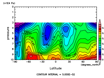
Figure 448: RH at Jun. by DCPAM
