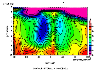
Figure 449: RH at Jun. by NCEP
