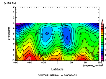
Figure 466: RH at Dec. by DCPAM
