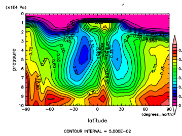
Figure 461: RH at Oct. by NCEP
