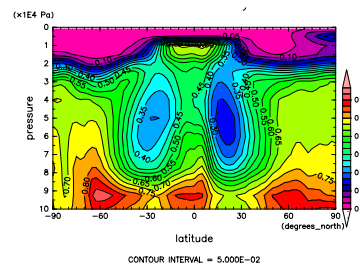
Figure 467: RH at Dec. by NCEP
