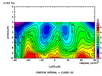
Figure 460: RH at Oct. by DCPAM
