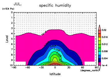
Figure 415: q at Jul. by DCPAM
