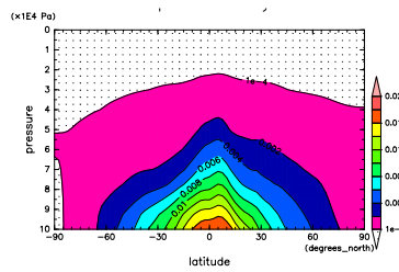
Figure 410: q at May by NCEP
