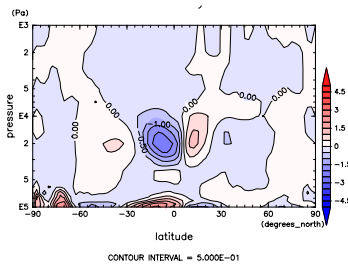
Figure 626: V at May by NCEP
