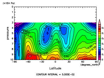
Figure 445: RH at May by DCPAM
