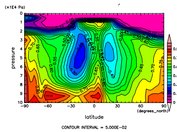
Figure 446: RH at May by NCEP
