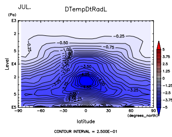
Figure 847: (\partial T / \partial t)_{LW} at Jul. by DCPAM by Figure 848: (\partial T / \partial t)_{LW} at Aug. by DCPAM
