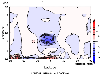
Figure 631: V at Jul. by DCPAM
