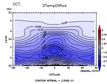
Figure 861: (\partial T/\partial t)_{SW+LW} at Sep. by DCPAM Figure 862: (\partial T/\partial t)_{SW+LW} at Oct. by DCPAM
