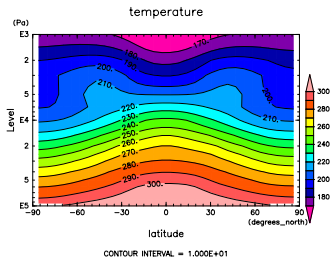
Figure 58: Annual mean T by DC-PAM
