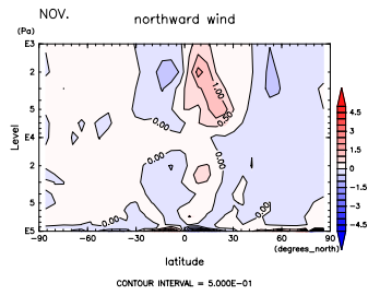
Figure 643: V at Nov. by DCPAM
