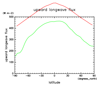
Figure 7: Annual average SLURA by DCPAM (red), NCEP (green)
