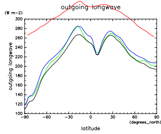
Figure 80: OLR at Aug. by DCPAM (red), NCEP (green), ECMWF (blue), and NOAA Interpolated OLR (black)
