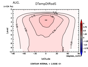
Figure 511: (\partial T/\partial t)_{SW} at Jul. by DCPAM Figure 512: (\partial T/\partial t)_{SW} at Aug. by DCPAM
