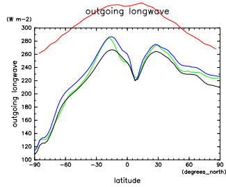
Figure 79: OLR at Jul. by DCPAM (red), NCEP (green), ECMWF (blue), and NOAA Interpolated OLR (black)
