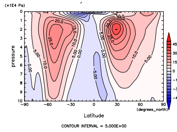
Figure 223: U at Mar. by DCPAM
