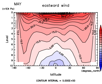
Figure 229: U at May by DCPAM
