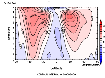
Figure 226: U at Apr. by DCPAM
