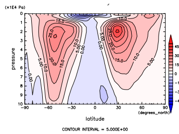
Figure 224: U at Mar. by NCEP
