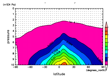
Figure 422: q at Sep. by NCEP
