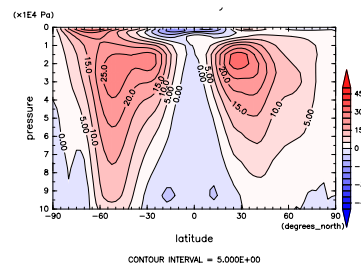
Figure 227: U at Apr. by NCEP
