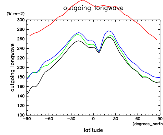
Figure 82: OLR at Oct. by DCPAM (red), NCEP (green), ECMWF (blue), and NOAA Interpolated OLR (black)
