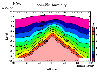
Figure 427: q at Nov. by DCPAM
