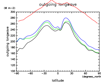
Figure 83: OLR at Nov. by DCPAM (red), NCEP (green), ECMWF (blue), and NOAA Interpolated OLR (black)
