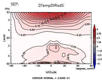
Figure 837: (\partial T/\partial t)_{sw} at Sep. by DCPAM
