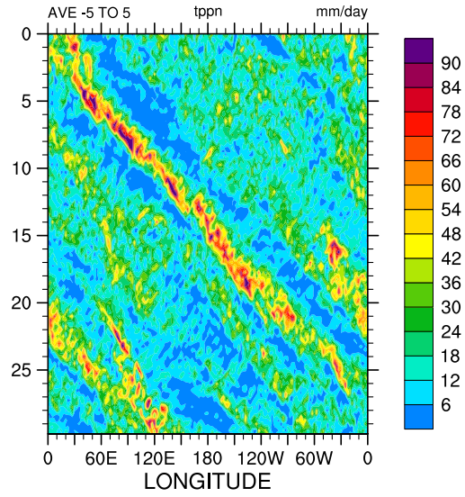
NICAM-04 - control (on 2.5° grid)
