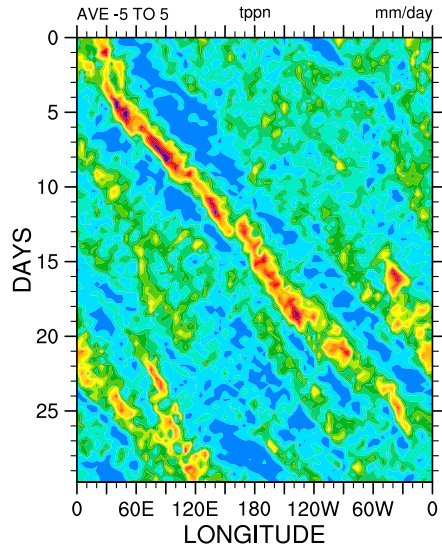
NICAM-04 - control (on 5° grid)
