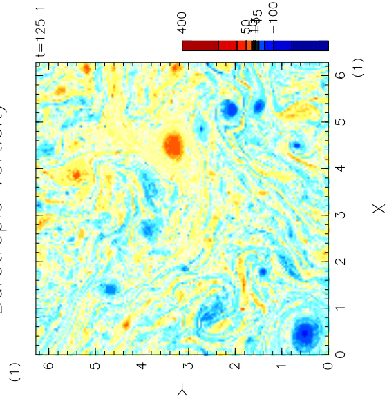
Barotropic Vorticity
