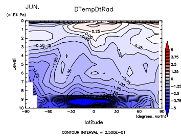
Figure 534: (\partial T / \partial t)_{SW+LW} at Jun. by DCPAM
