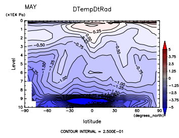
Figure 533: (\partial T / \partial t)_{SW+LW} at May by DCPAM
